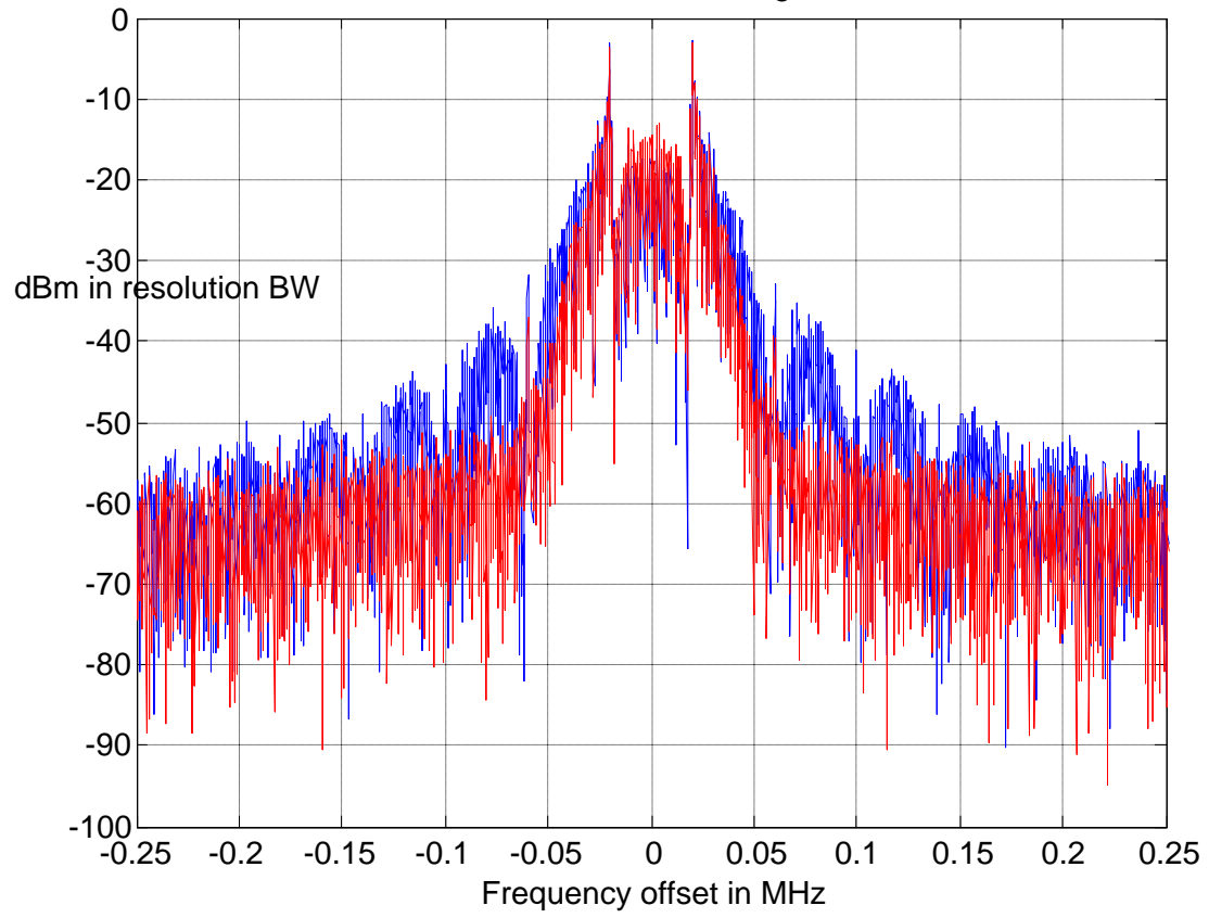
PSD of transmitted signal
