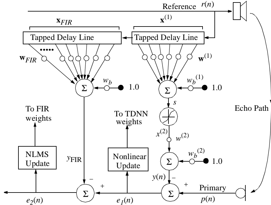
FIGURE 5. Proposed nonlinear AEC structure consists of a nonlinear tapped delay line neural network (TDNN) and linear FIR portions.
